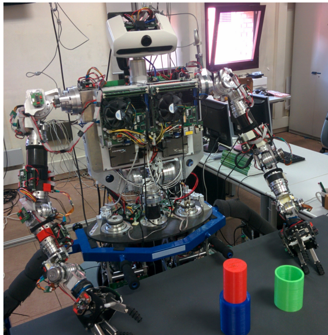
Figure 4.3: Humanoid robotics learning scenario: block-moving task.
