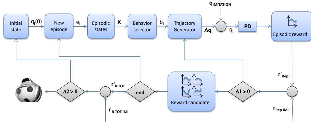
Figure 4.3: Overview of the innovation system. The process is very similar to Figure 4.2. The main difference appears in the trajectory generation. The generator perturbs the imitation trajectory q_{IMITATION} in an amount \Delta q_i , to generate a new trajectory q_i which is evaluated in terms of the episodic reward. The other difference is in the reward comparison \Delta_1 and \Delta_2 . In this case the objective is to maximize the difference. If the robot gets a better episodic reward r'_{Rep} than the reward obtained in the imitation r_{Rep IMI} , then \Delta_1 > 0 and the local optimization ends. If the robot gets a better reward r'_{R TOT} than the reward obtained in the imitation r_{R TOT IMI} , then \Delta_2 > 0 and the innovation is completed.
