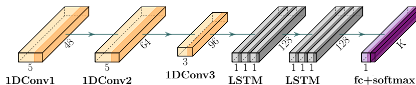
Fig. 3. Neural Network classification model.
